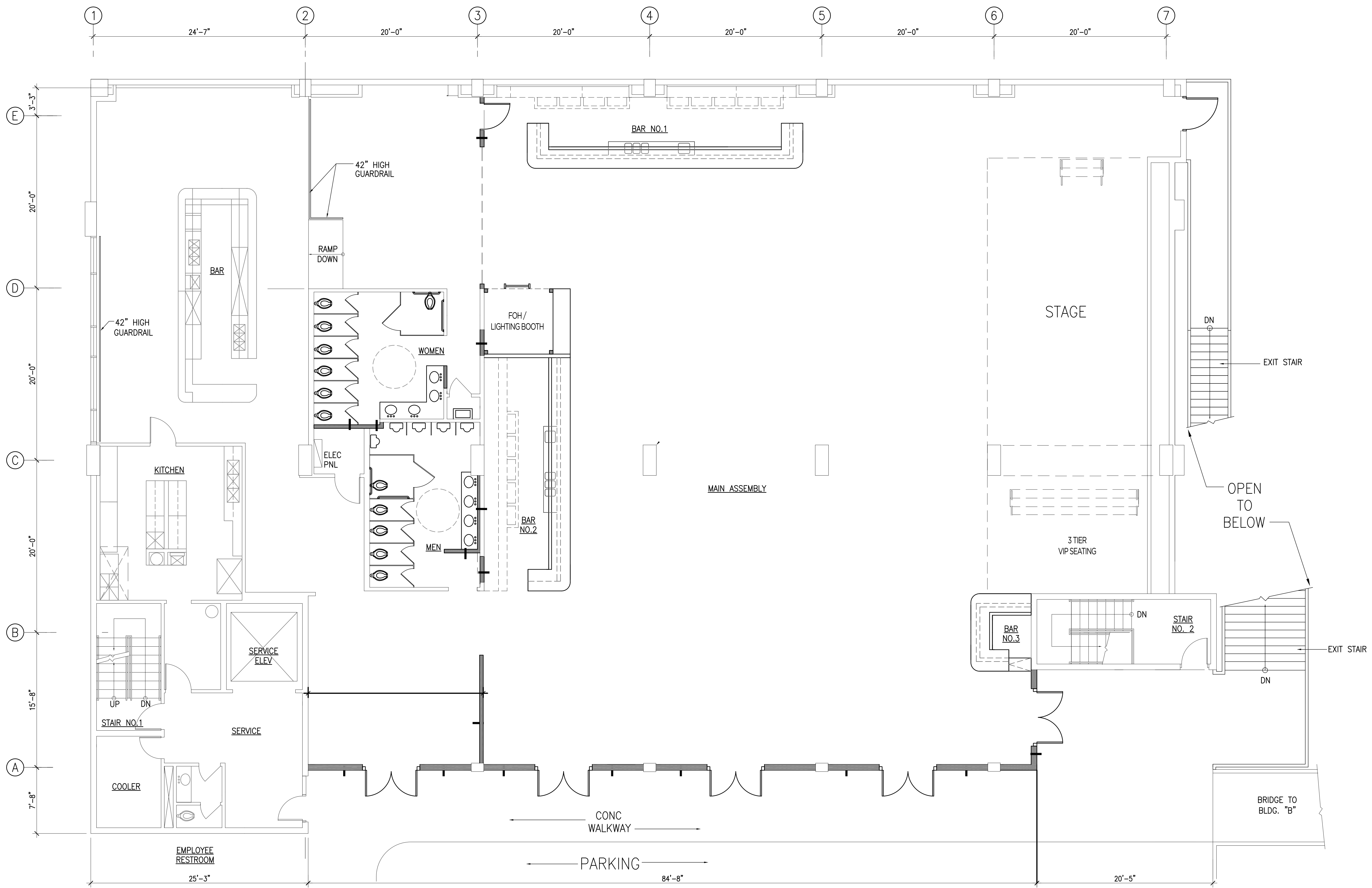
FLOOR PLAN EXIST BLDG. "A"
